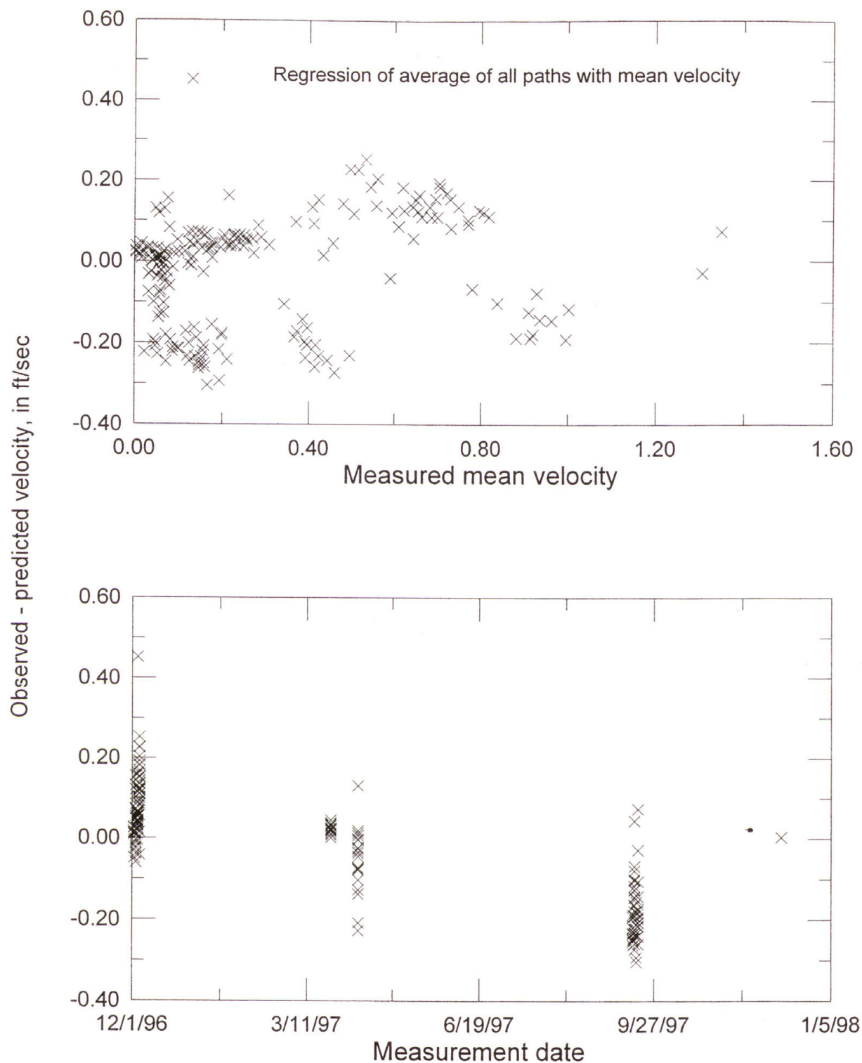
Figure 4.2-c - Graph showing differences between measured mean velocities and those predicted by rating based on average of all four AVM paths.
