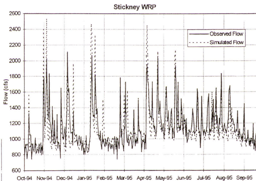
Figure 3.2-d - Comparison between simulated and observed flow at Stickney WRP for 1995.
