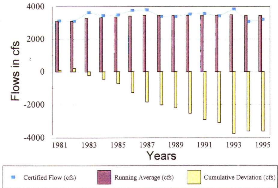
Figure 2.6-a: Illinois Lake Michigan diversion (1980 Modified Decree)
