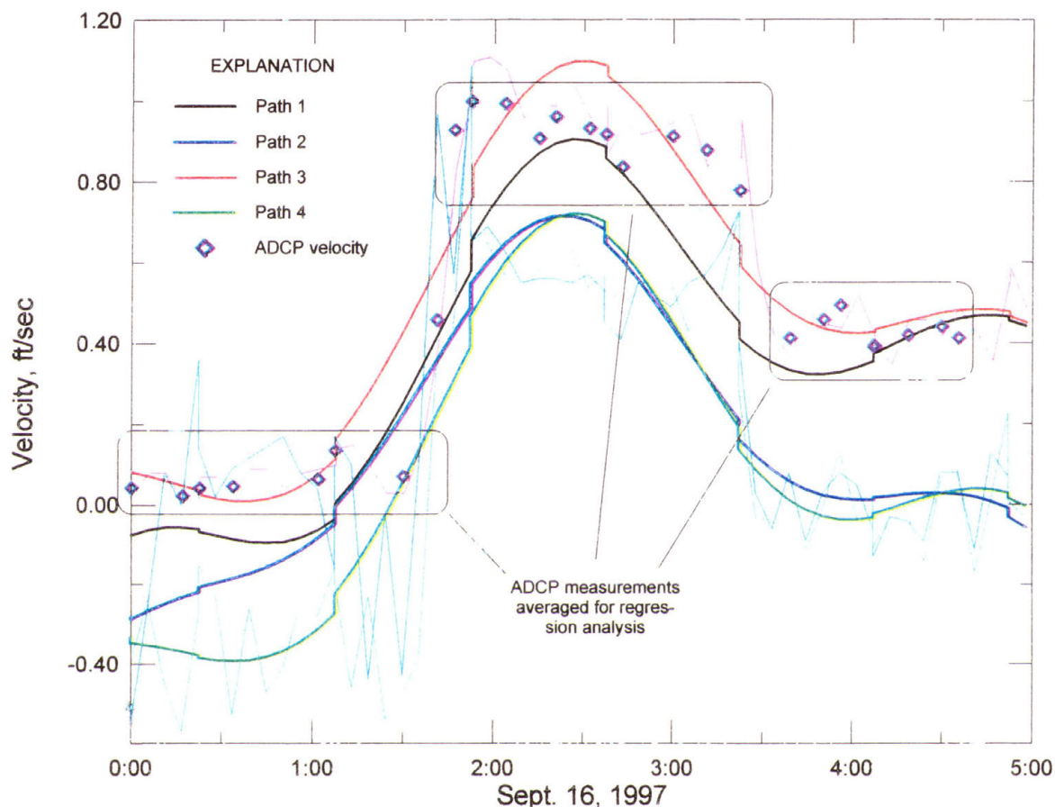
Figure 4.2-e - Graph showing measured and filtered AVM velocities and mean velocities from ADCP measurements at the Columbus Avenue AVM site, September 16, 1997.
