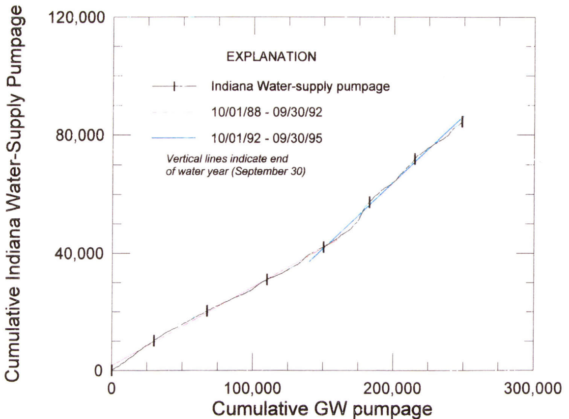
Figure 2.5-b: Double-mass-curve comparison of Indiana water-supply pumpage and groundwater pumpage discharged to the canal, water years 1989 through 1995.
