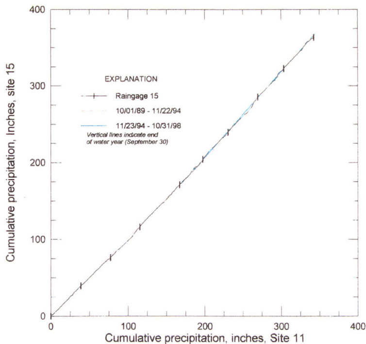
Figure 3.4-e - Double-mass curve comparing cumulative precipitation at sites 15 and 11, October 1, 1989 through September 30, 1998.
