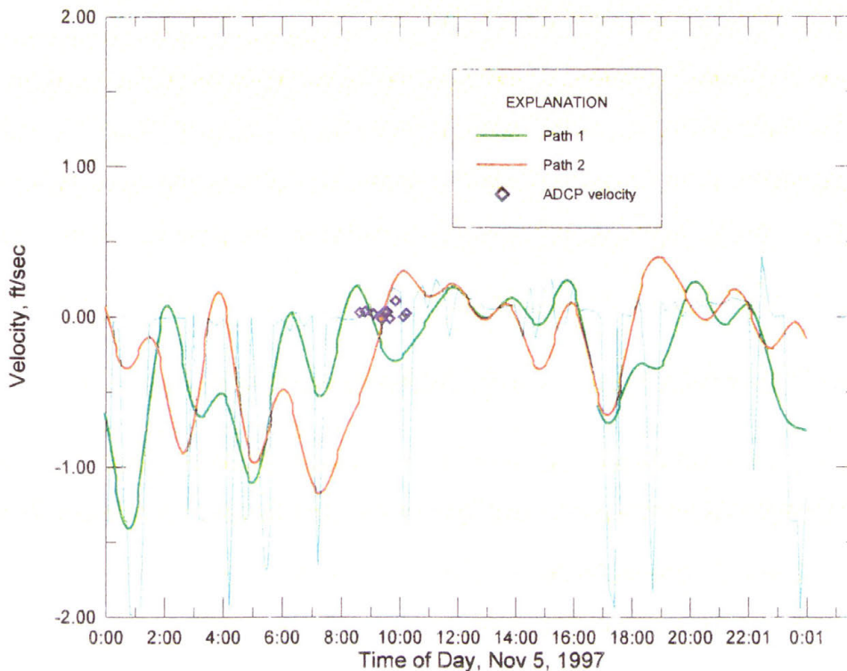
Figure 4.2-b - Graph showing measured and filtered AVM velocities and mean velocities from ADCP measurements at the O'Brien Locks and Dam AVM site, November 5, 1997.
