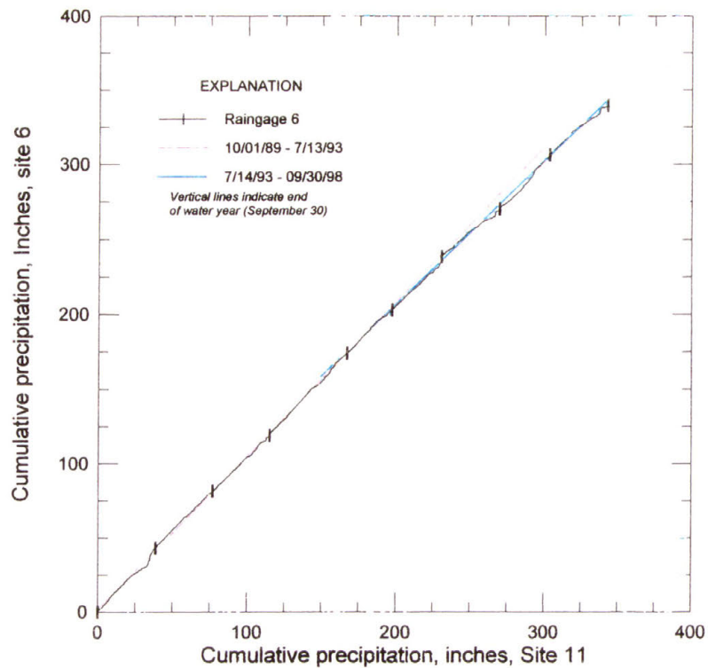
Figure 3.4-c - Double-mass curve comparing cumulative precipitation at sites 6 and 11, October 1, 1989 through September 30, 1998.
