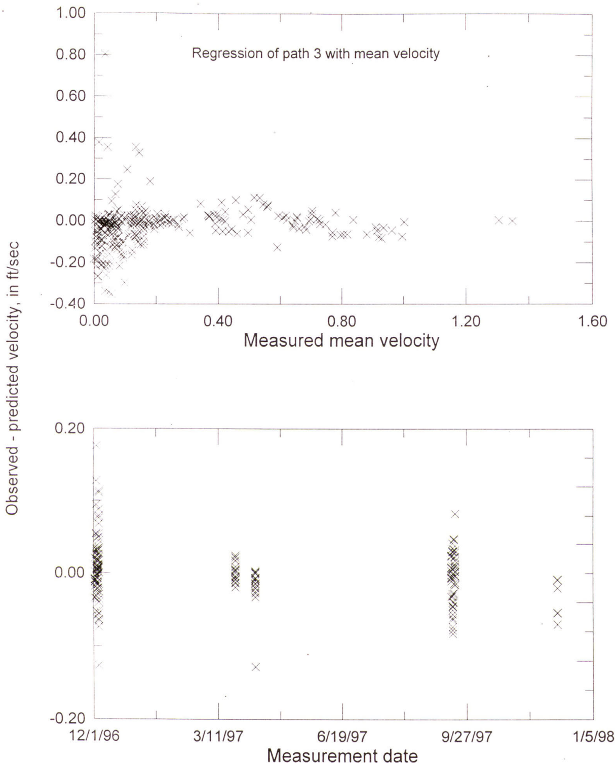
Figure 4.2-d - Graph showing differences between measured mean velocities and those predicted by rating based on AVM path 3.
