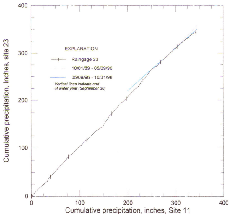
Figure 3.4-f - Double-mass curve comparing cumulative precipitation at sites 23 and 11, October 1, 1989 through September 30, 1998.
