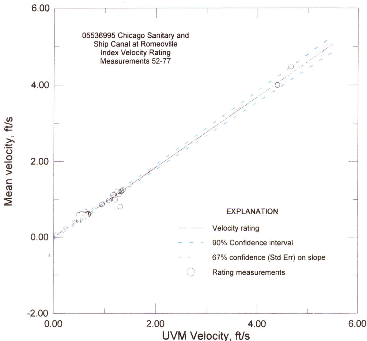
Figure 3.3-b - Index-velocity rating for Romeoville AVM.
