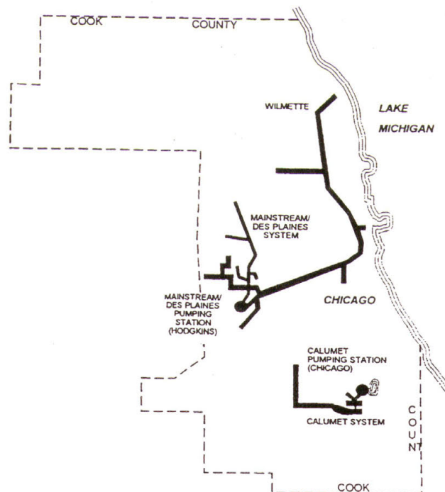
Figure 3.2-b - The Chicago TARP tunnels as of 1996.
