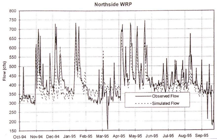
Figure 3.2-c - Comparison between simulated and observed flow at Northside WRP for 1995.
