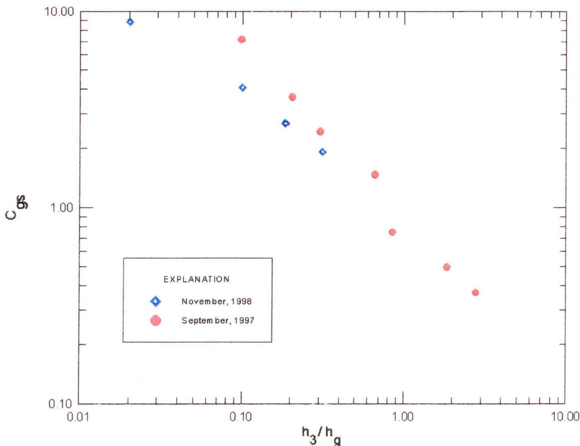
Figure 4.2-h - Discharge coefficients and gate openings for sluce-gates at the Chicago River Controlling Works.
