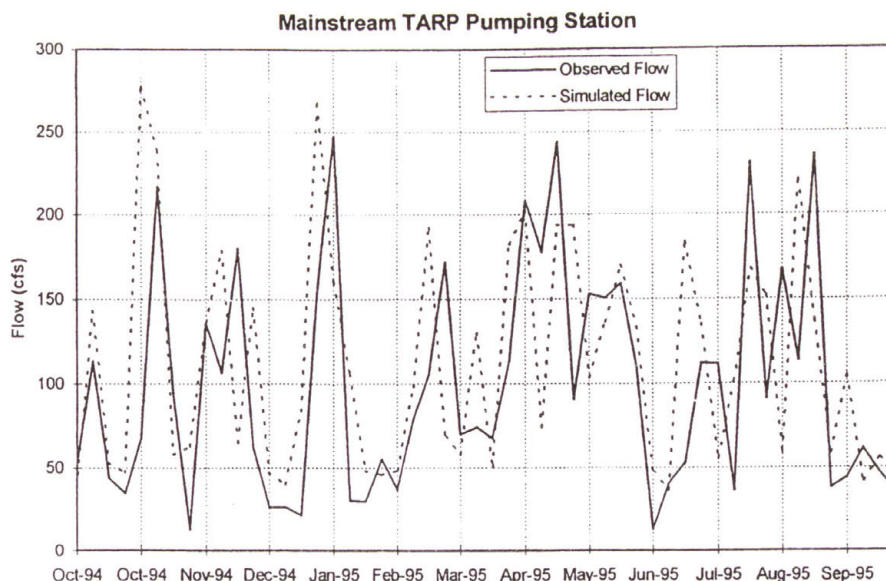
Figure 3.2-e - Comparison between simulated and observed flow at the Lemont WRP for 1995.
