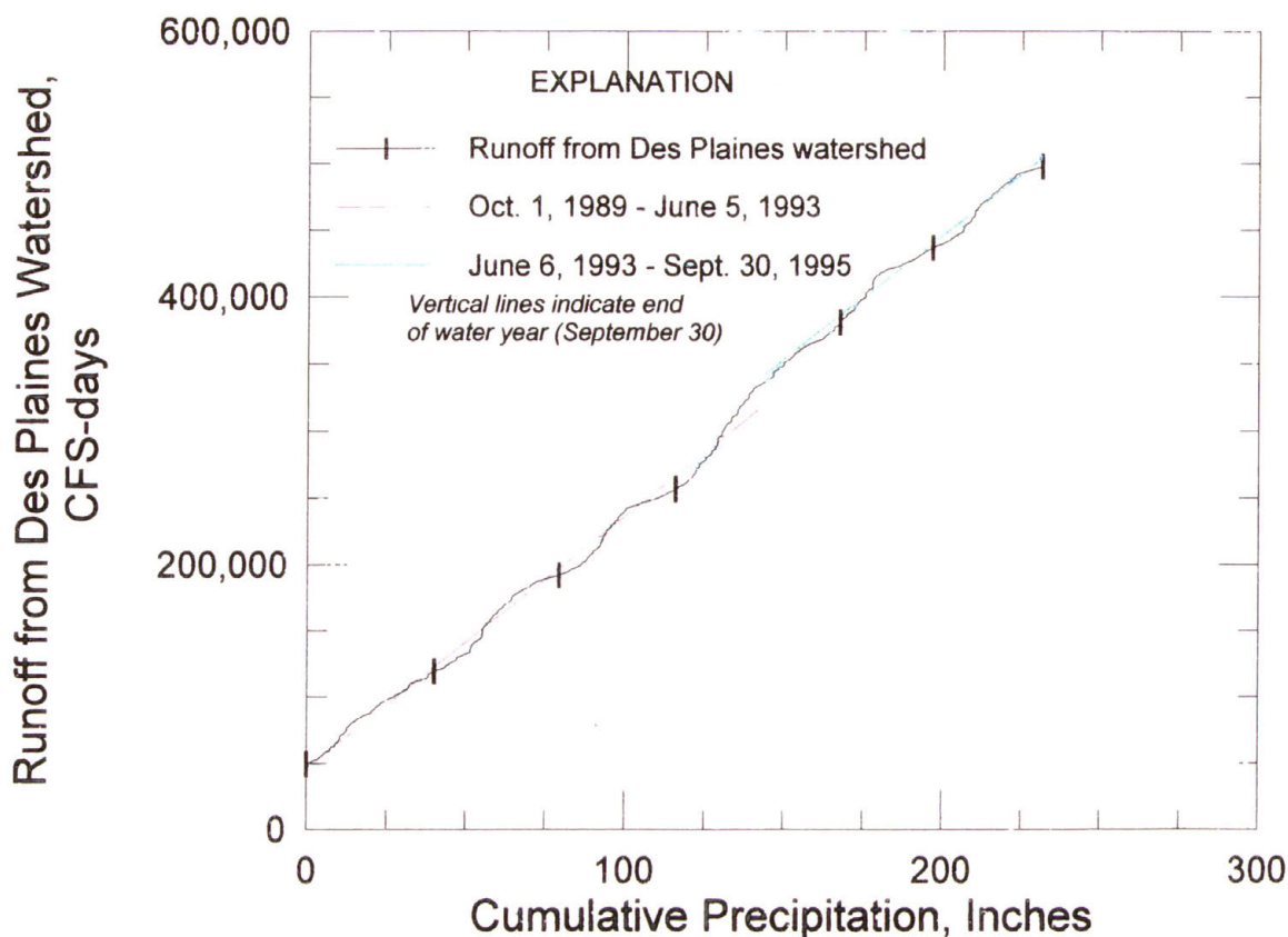
Figure 3.2-h - Double-mass-curve comparison of runoff from the Des Plaines River watershed reaching the canal and precipitation, water years 1990 through 1995.
