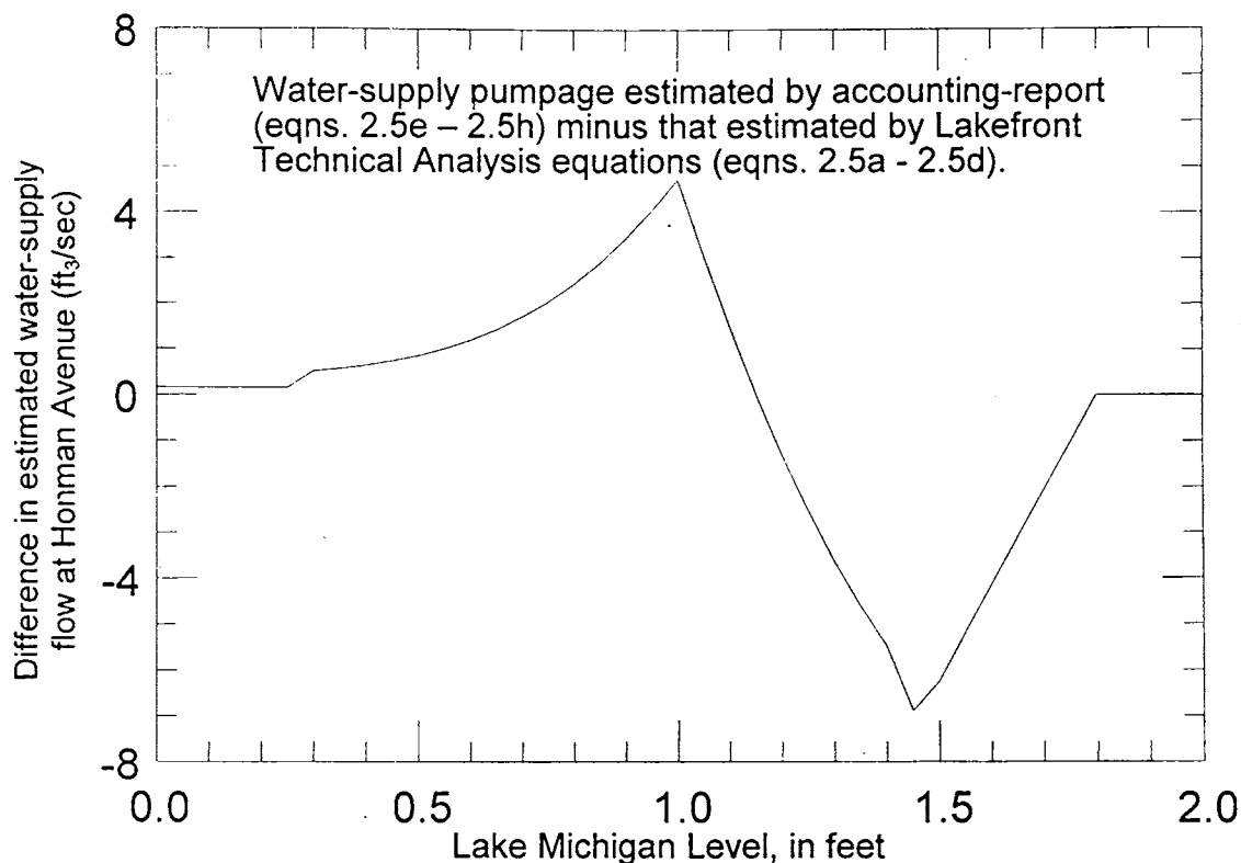
Figure 2.5-a: Differences in water-supply pumpage estimated by equations for diversion accounting and for Lakefront Accounting Technical Analysis
