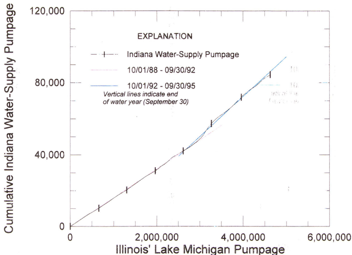
Figure 2.5-c: Double-mass-curve comparison of Indiana water-supply pumpage and Lake Michigan pumpage accountable to Illinois, water years 1989 through 1995.
