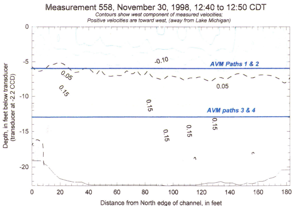
Figure 4.2-f - Graph showing west component of velocities from ADCP measurement 558 at the Columbus Avenue AVM site, November 30, 1998.
