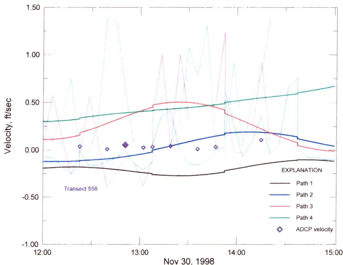
Figure 4.2-g - Graph showing measured and filtered AVM velocities and mean velocities from ADCP measurements at the Columbus Avenue AVM site, November 30, 1998.
