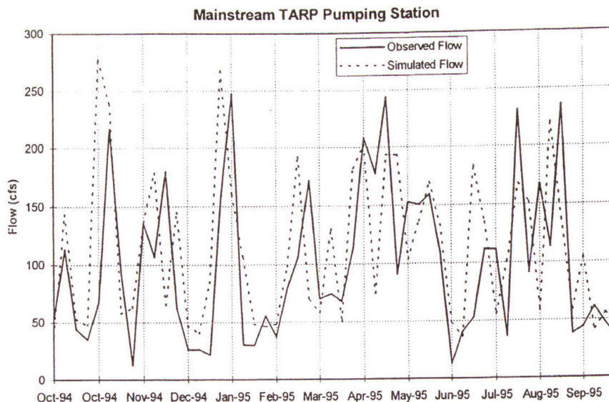
Figure 3.2-f - Comparison between simulated and observed flow at the Hodgkins (mainstream) TARP pumping station for 1995.
