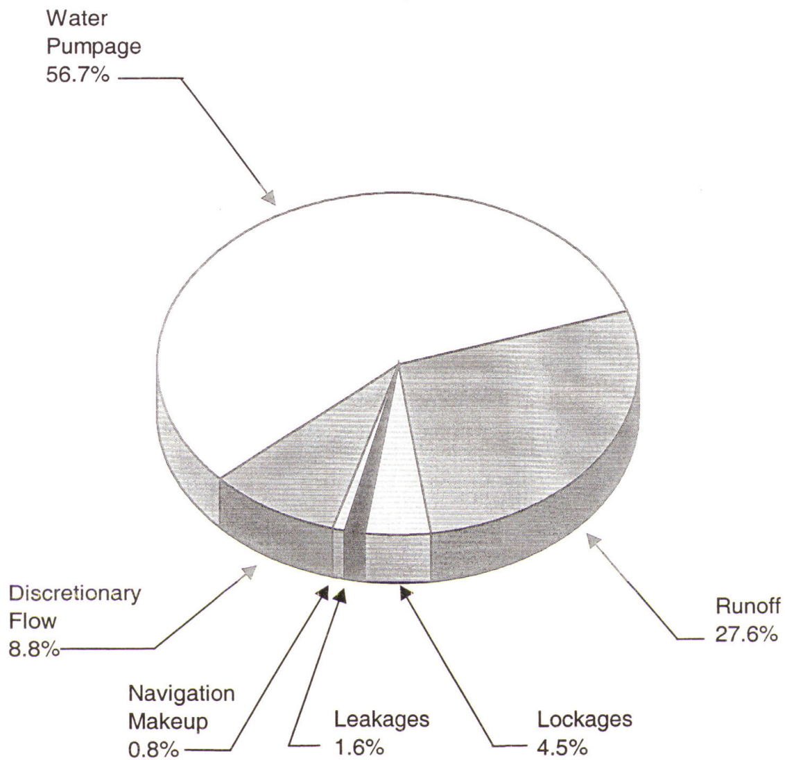
Figure 3 Component Breakdown of Illinois' Diversion Based Upon Columns 11 Through 13
