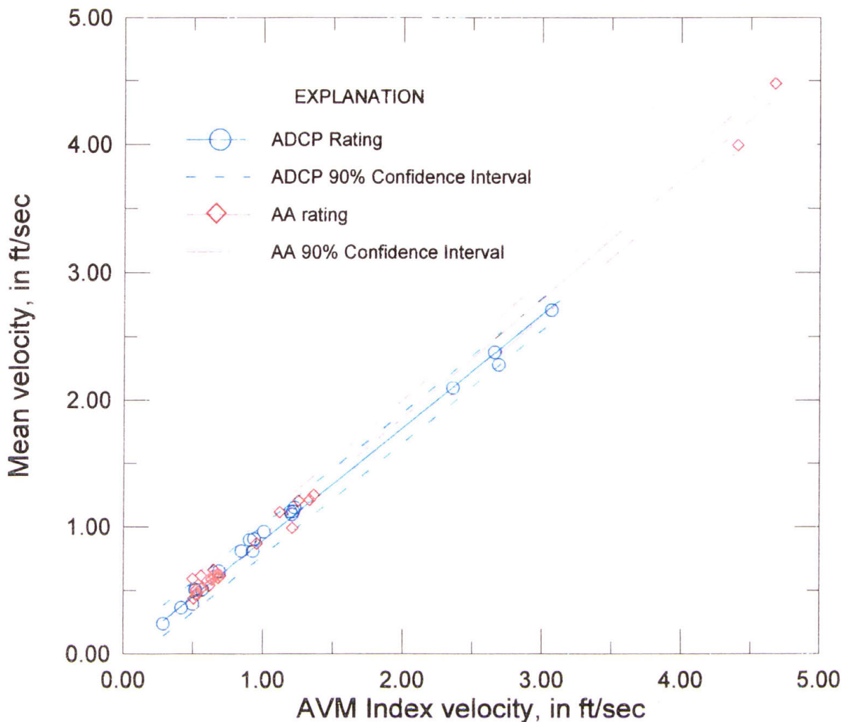
Figure 3.3-a - Graph showing ratings and 90-percent confidence intervals for index-velocity ratings developed from Price AA measurements and from ADCP measurements at Romeoville between November 1989 and October 1995.
