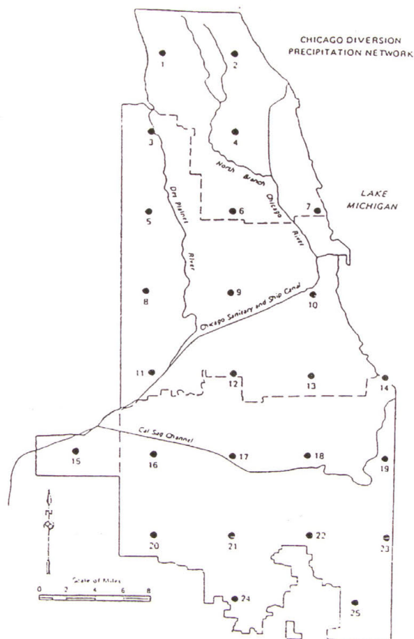
Figure 3.2-a - The 25-gage precipitation gage network.
