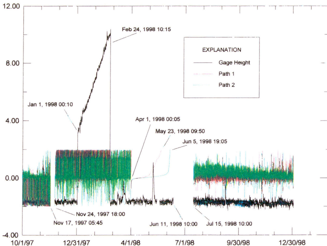
Figure 4.2-a - Record of water elevations and AVM velocities from the Calumet River at O'Brien Locks and Dam, October, 1997 through December, 1998.
