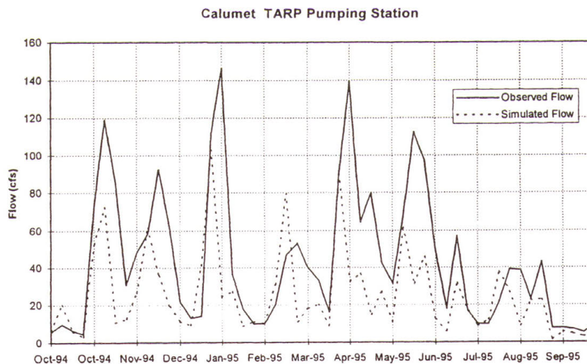
Figure 3.2-g - Comparison between simulated and observed flow at the Calumet pumping station for 1995.
