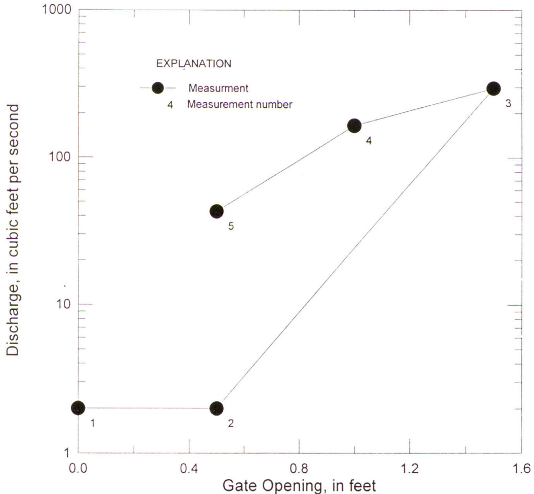
Figure 4.2-i - Discharges measured for different sluice-gate openings at the North Shore Channel at Wilmette, December 9, 1997.
