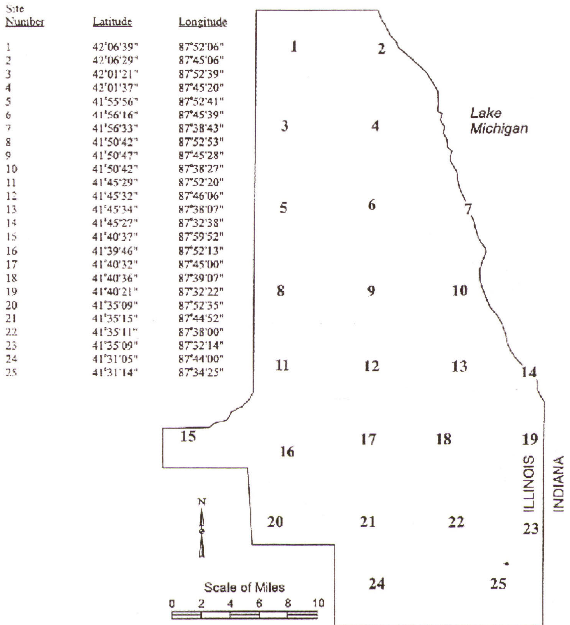
Figure 3.4-b - Configuration of the 25-site raingage network used during Water Years 1990-1993 (modified from Peppler, 1994).
