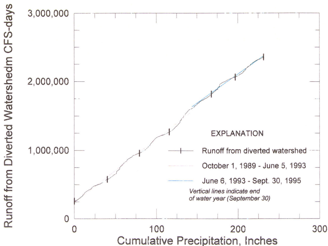
Figure 3.2-i - Double-mass-curve comparison of runoff from the diverted Lake Michigan watershed and precipitation, water years 1990 through 1995.
