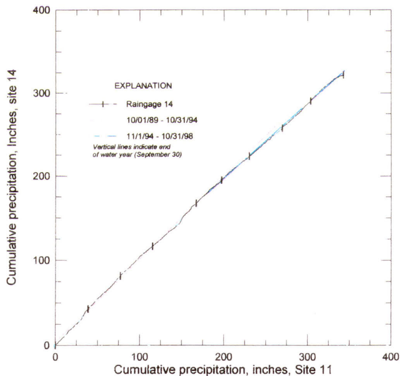
Figure 3.4-d - Double-mass curve comparing cumulative precipitation at sites 14 and 11, October 1, 1989 through September 30, 1998.
