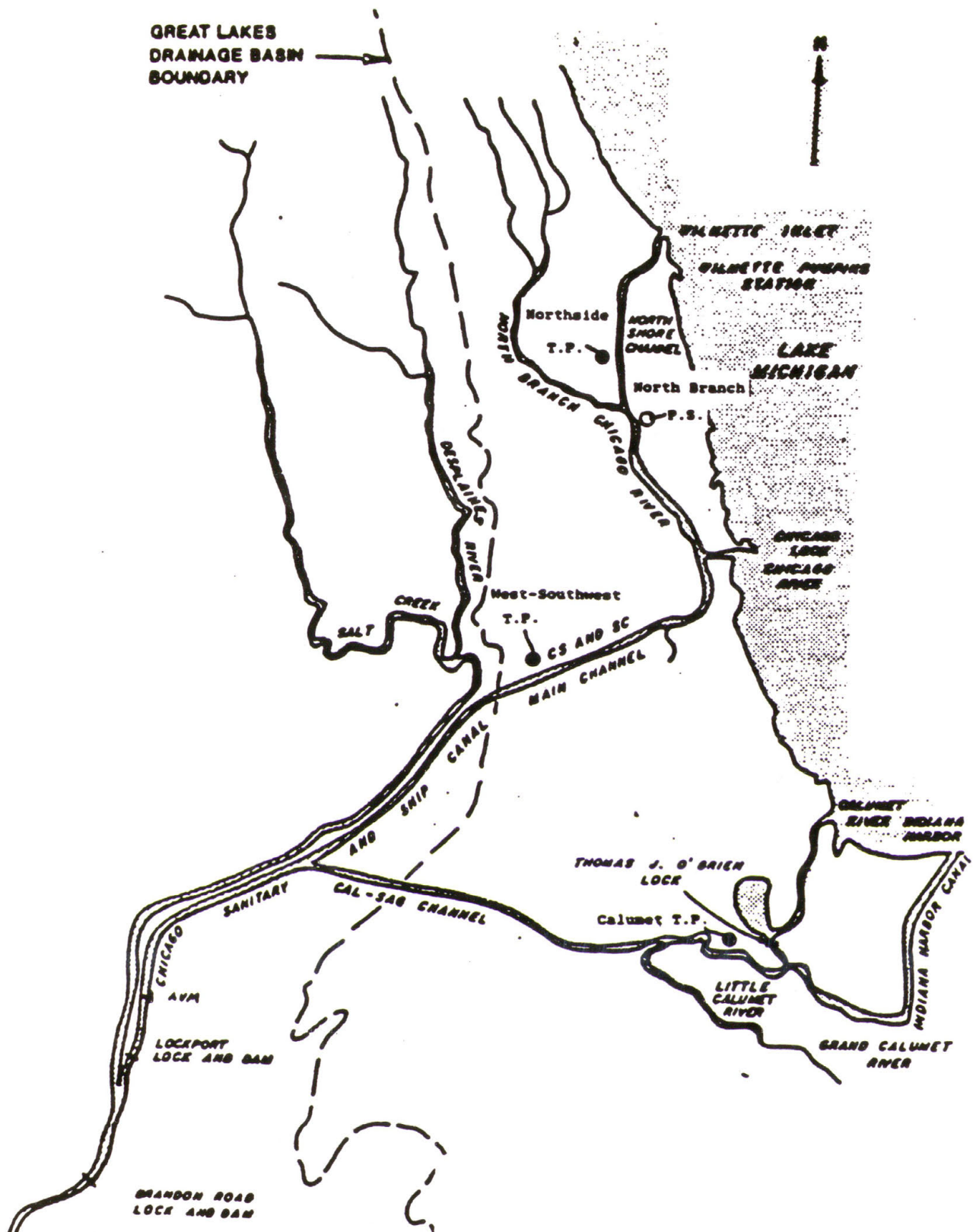
Figure 1-2 Lake Michigan Diversion at Chicago
