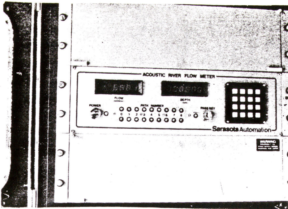
AVM Control panel
