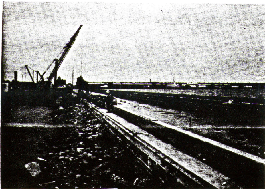
Figure 3-1 New parapet seal cutoff wall under construction
