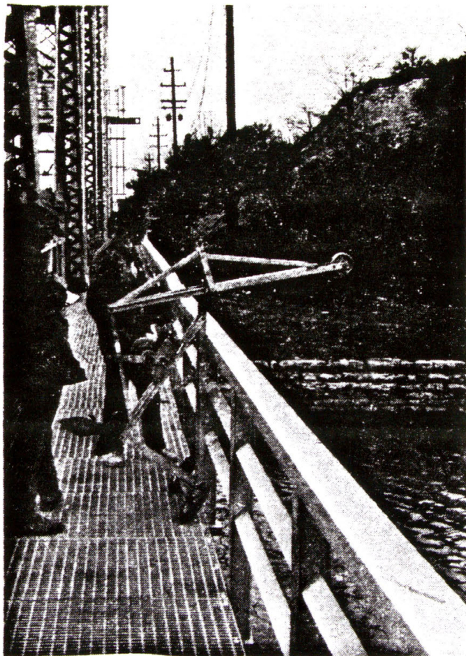
USGS velocity measurements near AVM site (mile, 296.1)
