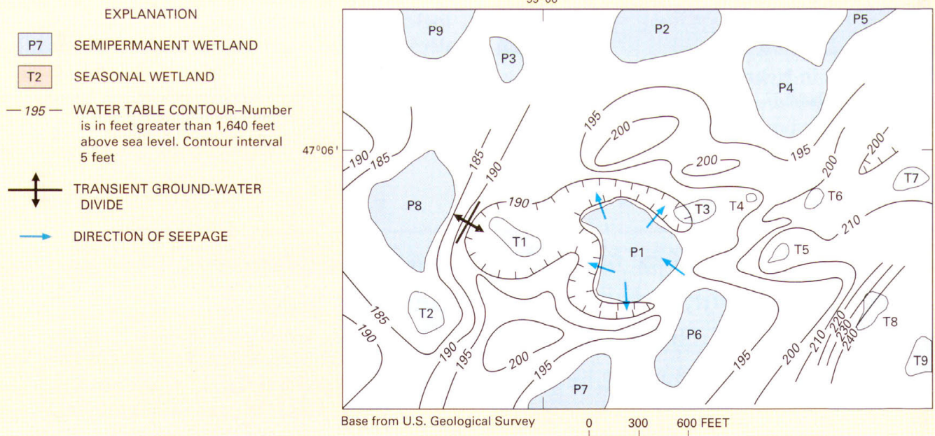
Figure K-1. Transpiration directly from ground water causes cones of depression to form by late summer around the perimeter of prairie pothole Wetland P1 in the Cottonwood Lake area in North Dakota. (Modified from Winter, T.C., and Rosenberry, D.O., 1995, The interaction of ground water with prairie pothole wetlands in the Cottonwood Lake area, east-central North Dakota, 1979–1990: Wetlands , v. 15, no. 3, p. 193–211.) (Used with permission.)
