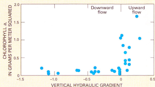
Figure F-1. Abundance of algae in streambed sediments, as indicated by concentration of chlorophyll a, was markedly greater in areas where water moved upward through the sediments than in areas where water moved downward through the sediments in Sycamore Creek in Arizona. (Modified from Valett, H.M., Fisher, S.G., Grimm, N.B., and Camill, P., 1994, Vertical hydrologic exchange and ecologic stability of a desert stream ecosystem: Ecology , v. 75, p. 548–560.) (Reprinted with permission.)
