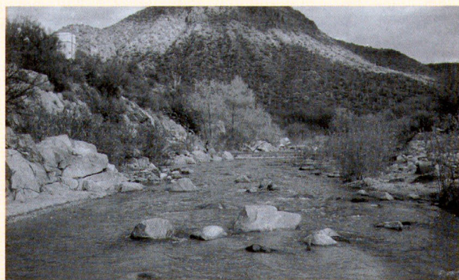
Sycamore Creek, Arizona. (Photograph by Owen Baynham.)
