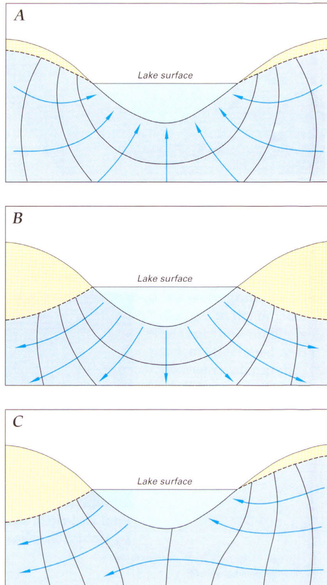
Figure 16. Lakes can receive ground-water inflow (A), lose water as seepage to ground water (B), or both (C).
