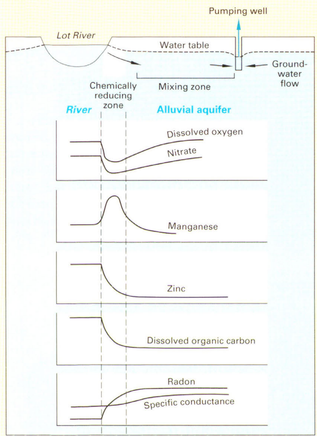
Figure G-2. Sharp changes in chemical concentrations were detected over short distances as water from the Lot River in France moved into its contiguous alluvial aquifer in response to pumping from a well. Specific conductance of water was used as an environmental tracer to determine the extent of mixing of surface water with ground water, and radon was used to determine the inflow rate of stream water. Both pieces of information were then used to calculate the rate at which dissolved metals reacted to form solid phases during movement of stream water toward the pumping well. (Modified from Bourg, A.C.M., and Bertin, C., 1993, Biogeochemical processes during the infiltration of river water into an alluvial aquifer: Environmental Science and Technology , v. 27, p. 661–666.) (Reprinted with permission from the American Chemical Society.)
