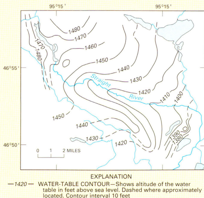
Figure I-1. Small streams, such as the Straight River in Minnesota, commonly do not have flood plains. The flow of ground water directly into the river is indicated by the water-table contours that bend sharply upstream. (Modified from Stark, J.R., Armstrong, D.S., and Zwilling, D.R., 1994, Stream-aquifer interactions in the Straight River area, Becker and Hubbard Counties, Minnesota: U.S. Geological Survey Water-Resources Investigations Report 94-4009 , 83 p.)
