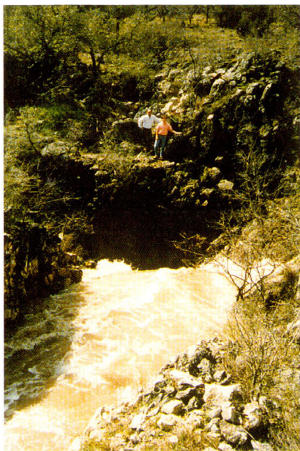
Stream disappearing into sink-hole in karst terrain in Texas. (Photograph by Jon Gilhousen.)
