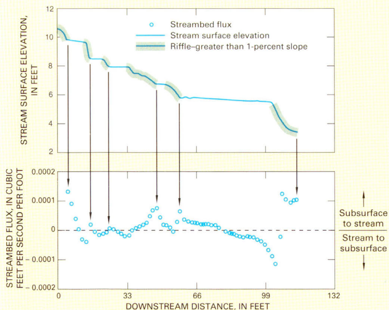
Figure H-2. In mountain streams characterized by pools and riffles, such as at Saint Kevin Gulch in Colorado, inflow of water from the hyporheic zone to the stream was greatest at the downstream end of riffles. (Modified from Harvey, J.W., and Bengala, K.E., 1993, The effect of streambed topography on surface-subsurface water exchange in mountain catchments: Water Resources Research , v. 29, p. 89–98.)
