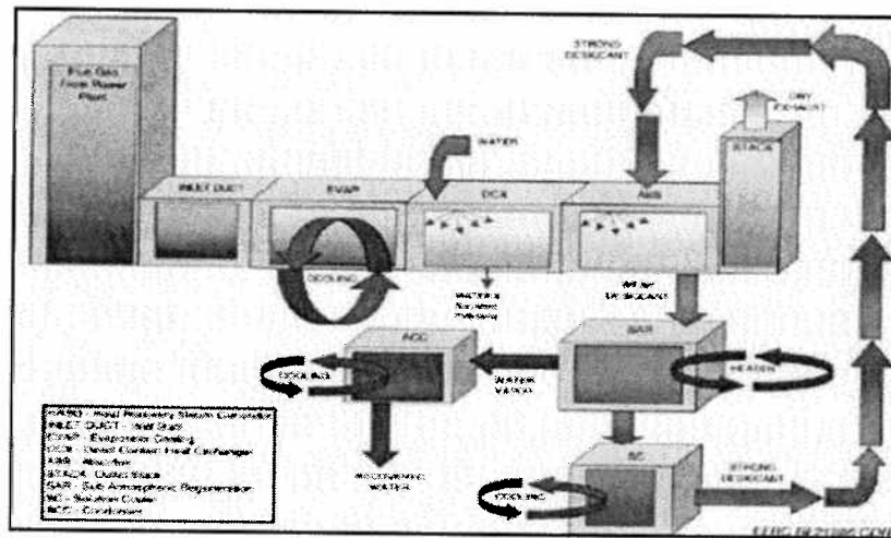
Figure 4 - Conceptual Design of Liquid Desiccant Process
