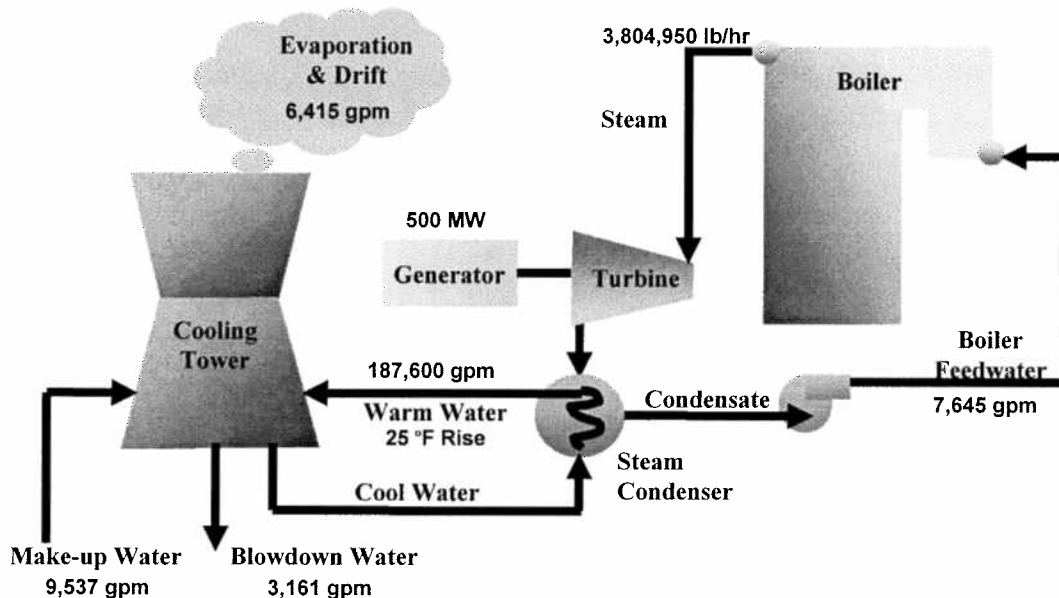
Figure 3 - Process Flow Schematic for Wet Recirculating Cooling Water System
