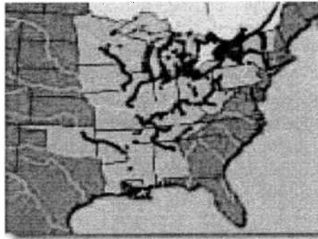
Figure 6 - North America Distribution of Zebra Mussels
