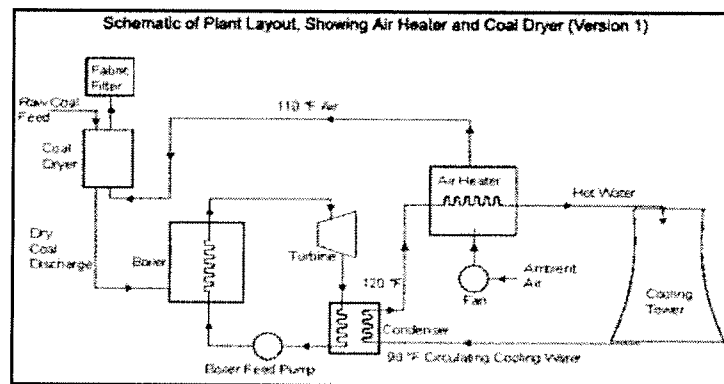
Figure 5 - Schematic of Plant Layout
