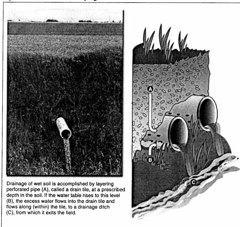
Figure 3: Drain Tile Conveying Water from a Field
