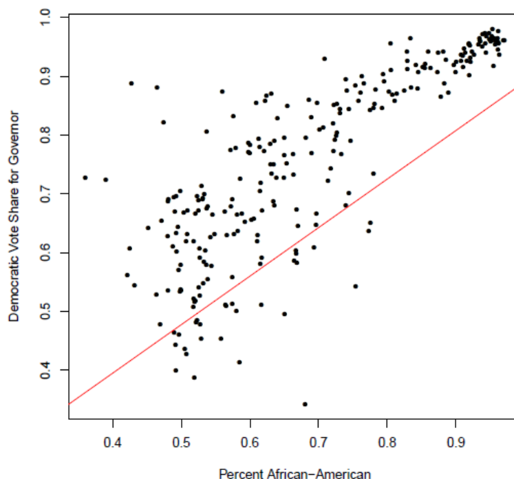
Figure 1: The correlation between BVAP and Democratic vote share in the Challenged District VTDs is 0.81.
