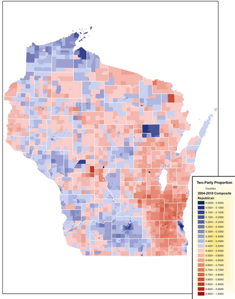
Gimpel Figure 3 2004-2010 Statewide Elections Two-Party Proportion
