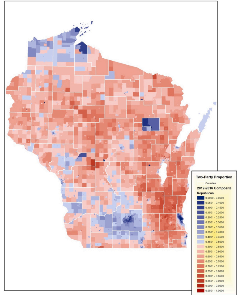
Gimpel Figure 4 2012-2016 Statewide Elections Two-Party Proportion
